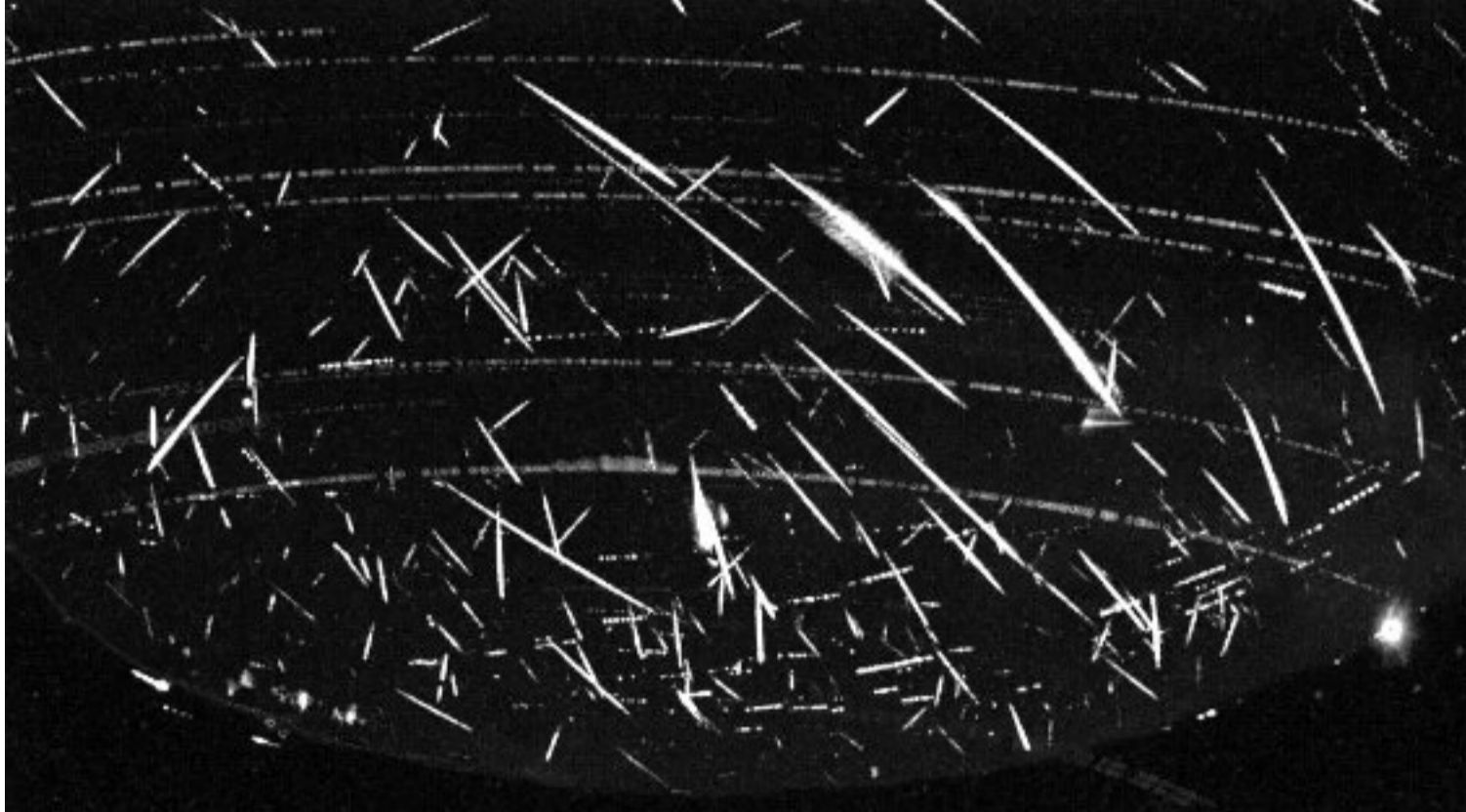
Meteor data from a single night, composed onto a single image.
